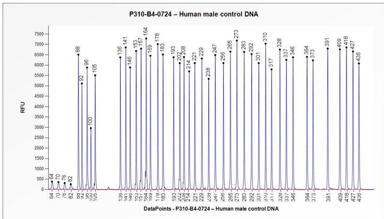
Figure 1. Capillary electrophoresis pattern from a sample of approximately 50 ng human male control DNA analysed with SALSA MLPA Probemix P310 TCOF1 (B4-0724).
