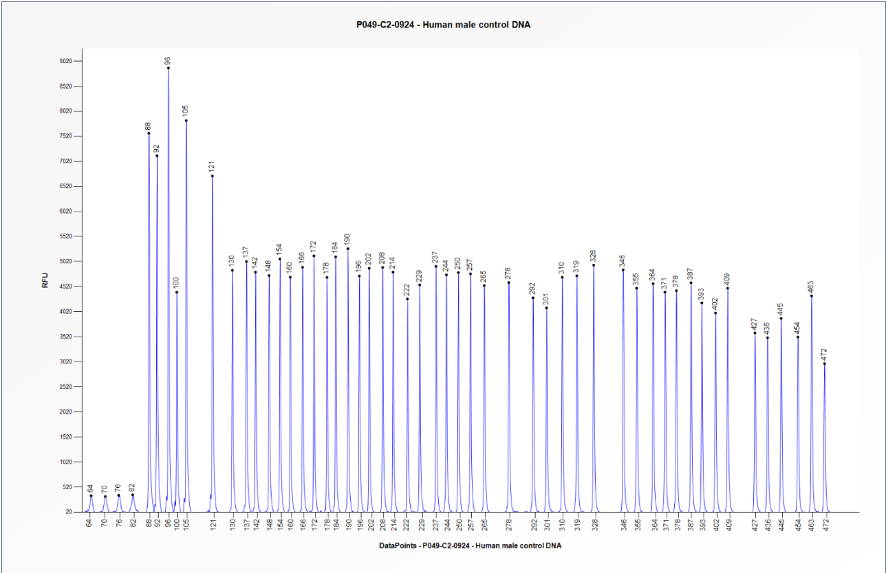
Figure 1. Capillary electrophoresis pattern from a sample of approximately 50 ng human male control DNA analysed with SALSA MLPA Probemix P049 SLC6A8-ABCD1 (C2-0924).
