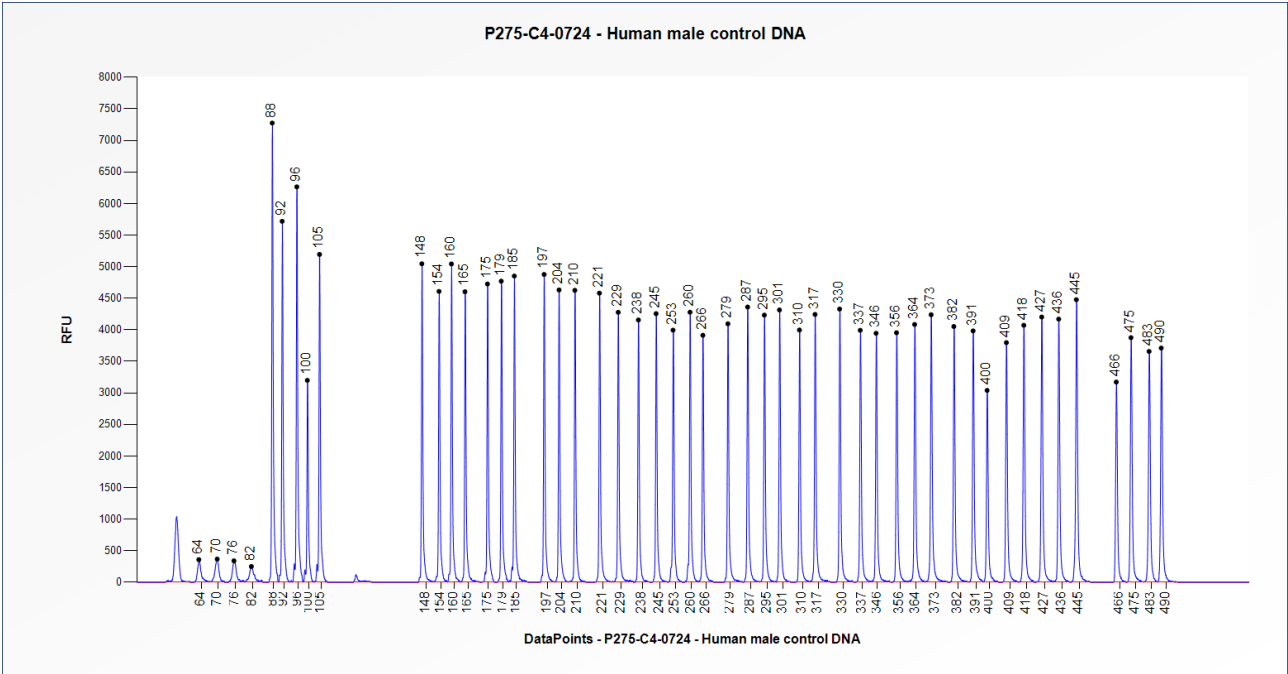
Figure 1. Capillary electrophoresis pattern from a sample of approximately 50 ng human male control DNA analysed with SALSA MLPA Probemix P275 MAPT GRN (C4-0724).
