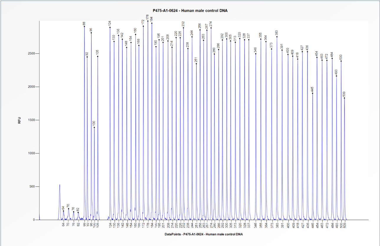
Figure 1. Capillary electrophoresis pattern from a sample of approximately 50 ng human male control DNA analysed with SALSA MLPA Probemix P475 FOXP1 - FOXP2 (A1-0624).
