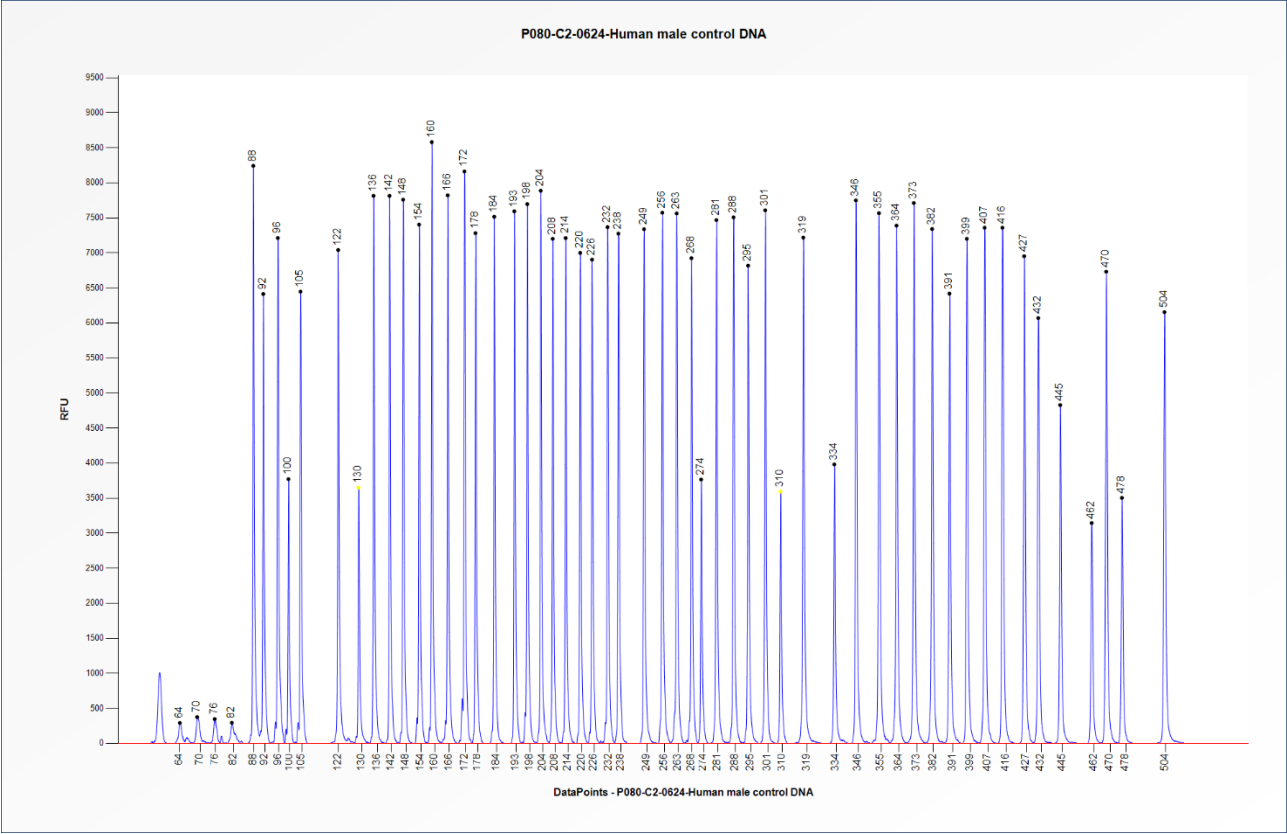
Figure 1. Capillary electrophoresis pattern from a sample of approximately 50 ng human male control DNA analysed with SALSA MLPA Probemix P080 Craniofacial (C2-0624).
