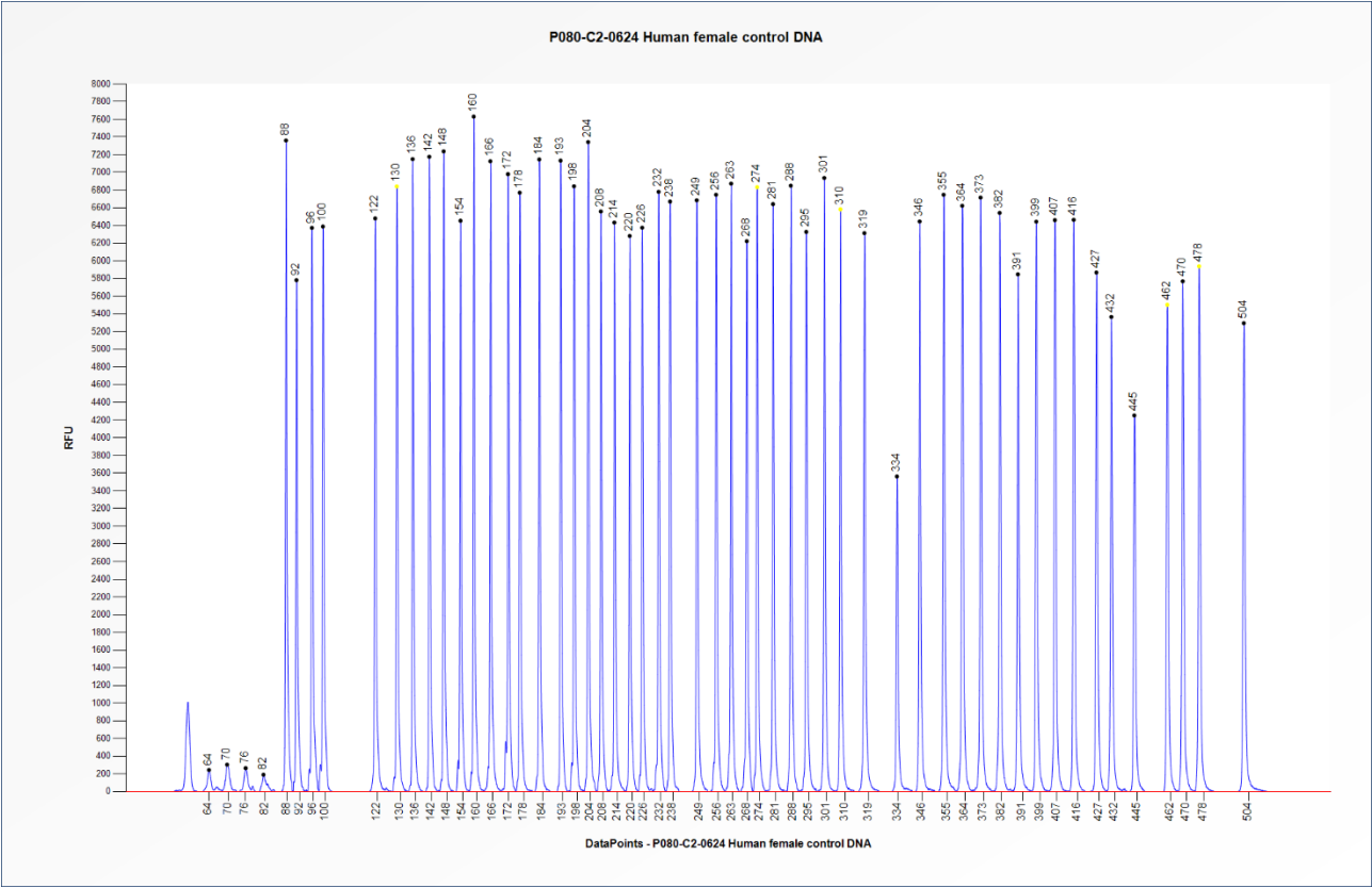
Figure 2. Capillary electrophoresis pattern from a sample of approximately 50 ng human female control DNA analysed with SALSA MLPA Probemix P080 Craniofacial (C2-0624).
