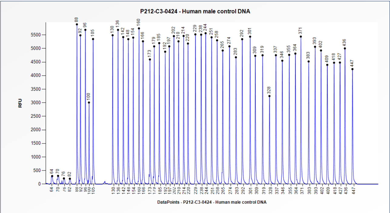
Figure 1. Capillary electrophoresis pattern from a sample of approximately 50 ng human male control DNA analysed with SALSA MLPA Probemix P212 DBA (C3-0424).
