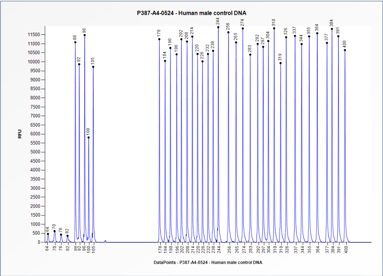
Figure 1. Capillary electrophoresis pattern from a sample of approximately 50 ng human male control DNA analysed with SALSA MLPA Probemix P387 NPHP1 (A4-0524).
