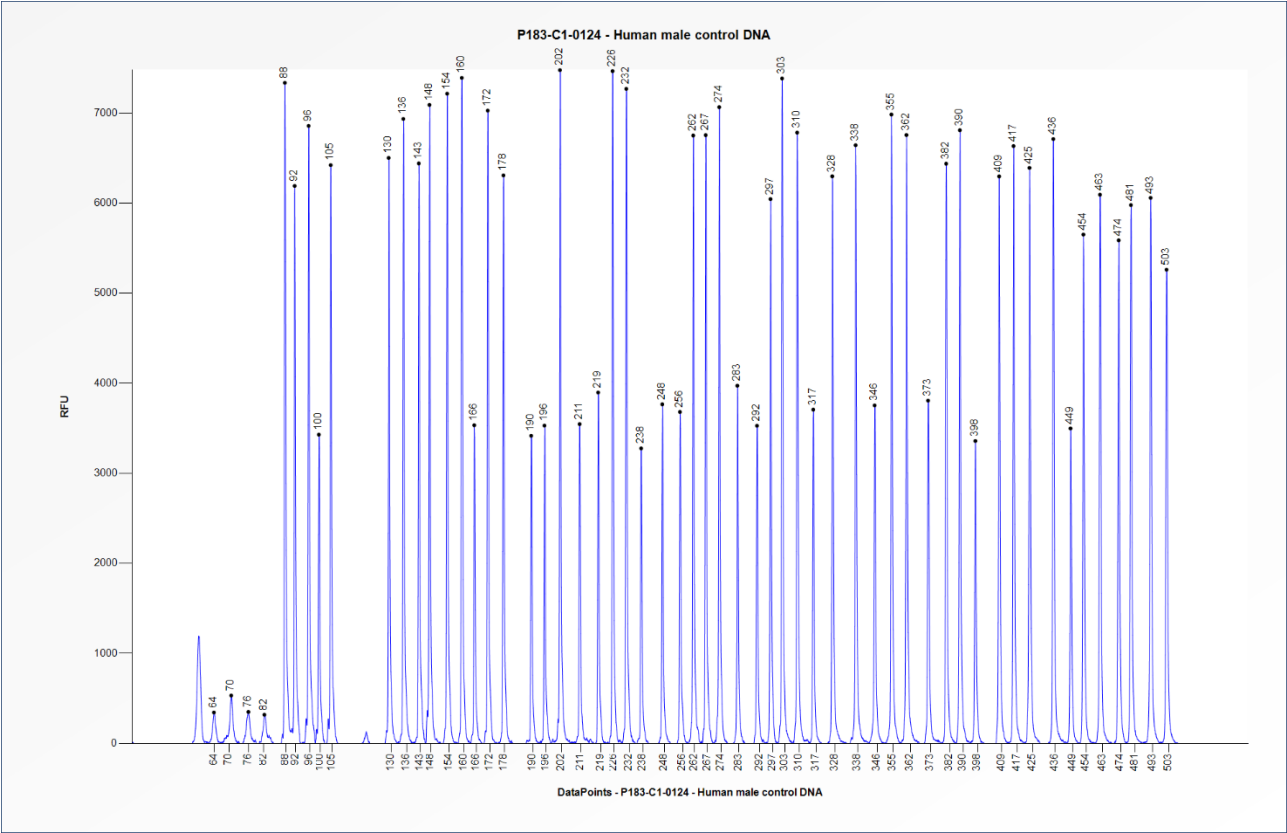
Figure 1. Capillary electrophoresis pattern from a sample of approximately 50 ng human male control DNA analysed with SALSA MLPA Probemix P183 EDA-EDAR-EDARADD (C1-0124).
