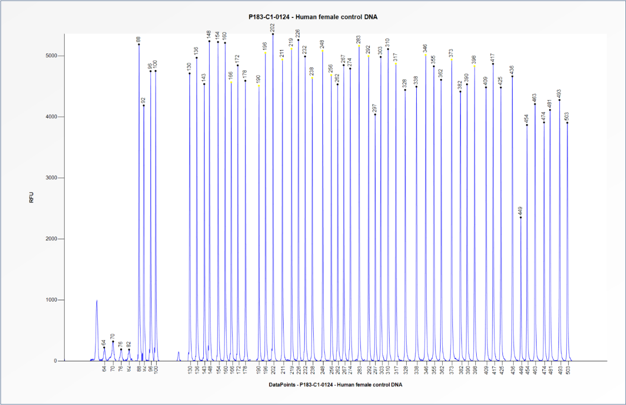
Figure 2. Capillary electrophoresis pattern from a sample of approximately 50 ng human female control DNA analysed with SALSA MLPA Probemix P183 EDA-EDAR-EDARADD (C1-0124).
