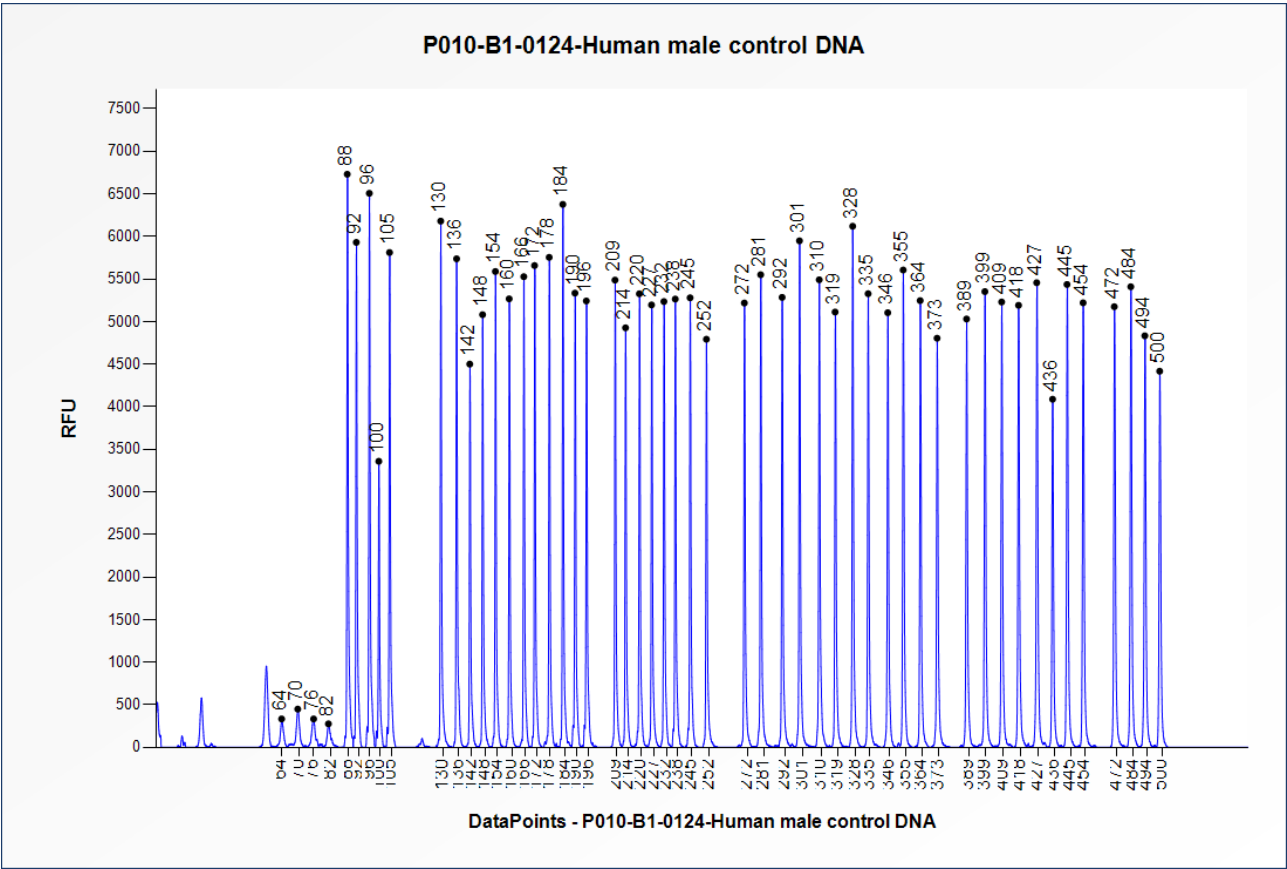
Figure 1. Capillary electrophoresis pattern from a sample of approximately 50 ng human male control DNA analysed with SALSA MLPA Probemix P010 POLG (B1-0124).
