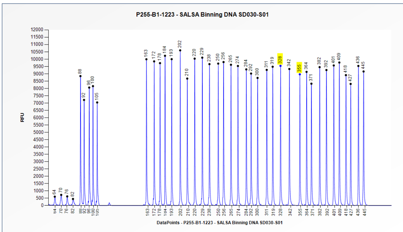
Figure 2. Capillary electrophoresis pattern from SALSA Binning DNA SD030-S01 (approximately 50 ng) analysed with SALSA MLPA Probemix P255-B1 ALDOB-FBP1 (B1-1223). The location of the ALDOB A149P (c.448G>C) and the ALDOB A174D (c.524C>A) mutation specific probes, at 328 nt and 355 nt respectively, are indicated.
