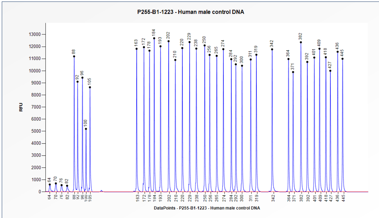
Figure 1. Capillary electrophoresis pattern from a sample of approximately 50 ng human male control DNA analysed with SALSA MLPA Probemix P255-B1 ALDOB-FBP1 (B1-1223).
