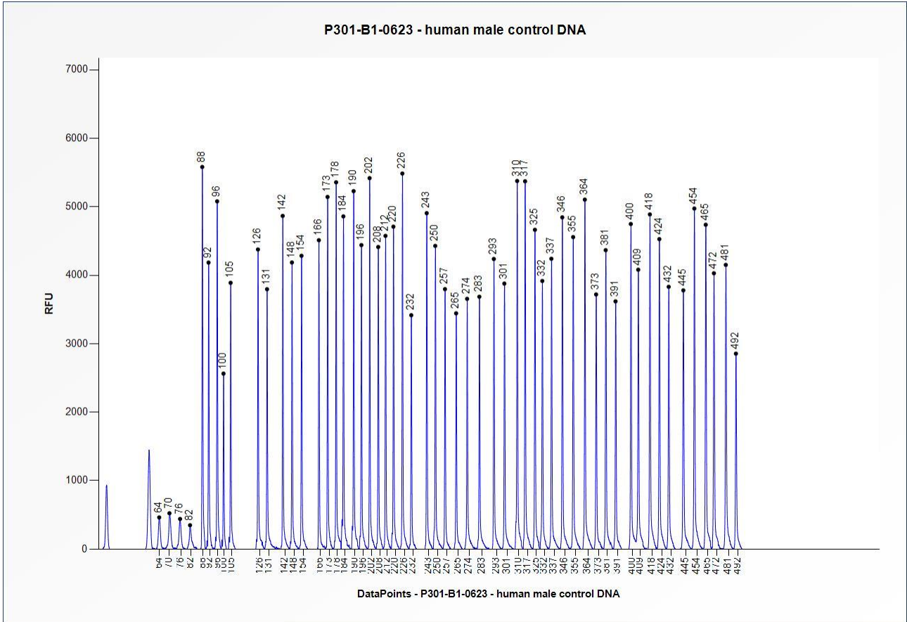
Figure 1. Capillary electrophoresis pattern from a sample of approximately 50 ng human male control DNA analysed with SALSA MLPA Probemix P301-B1 Medulloblastoma mix 1 (B1-0623).
