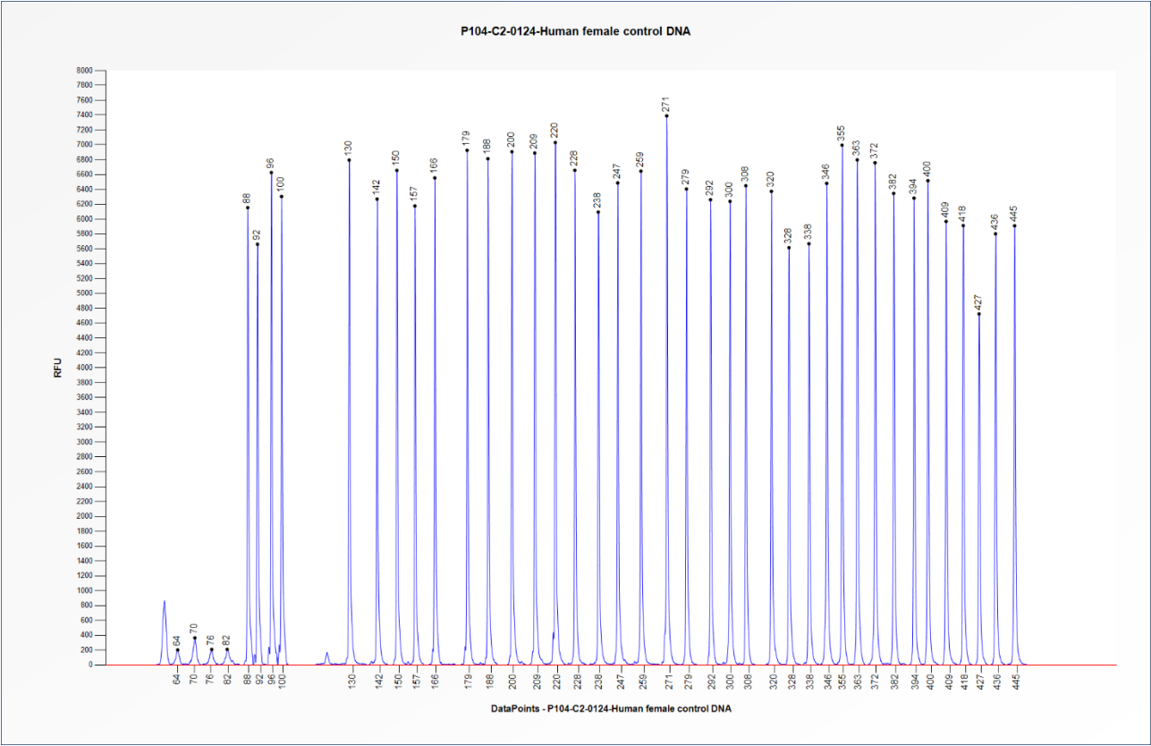
Figure 2. Capillary electrophoresis pattern from a sample of approximately 50 ng human female control DNA analysed with SALSA MLPA Probemix P104 Menkes ATP7A (C2-0124).
