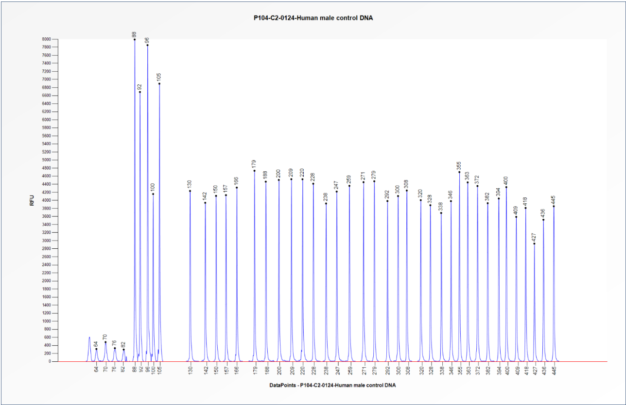
Figure 1. Capillary electrophoresis pattern from a sample of approximately 50 ng human male control DNA analysed with SALSA MLPA Probemix P104 Menkes ATP7A (C2-0124).
