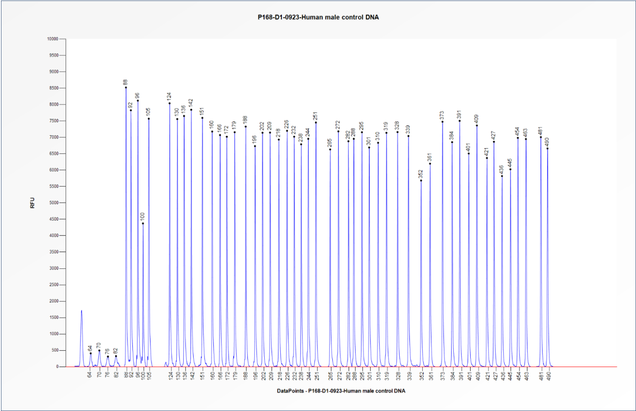
Figure 1. Capillary electrophoresis pattern from a sample of approximately 50 ng human male control DNA analysed with SALSA MLPA Probemix P168 ARVC-PKP2 (D1-0923).
