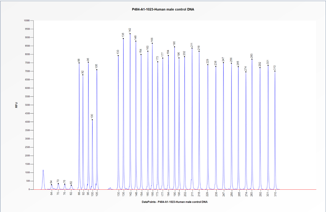
Figure 1. Capillary electrophoresis pattern from a sample of approximately 50 ng human male control DNA analysed with SALSA MLPA Probemix P484 ALPL (A1-1023).
