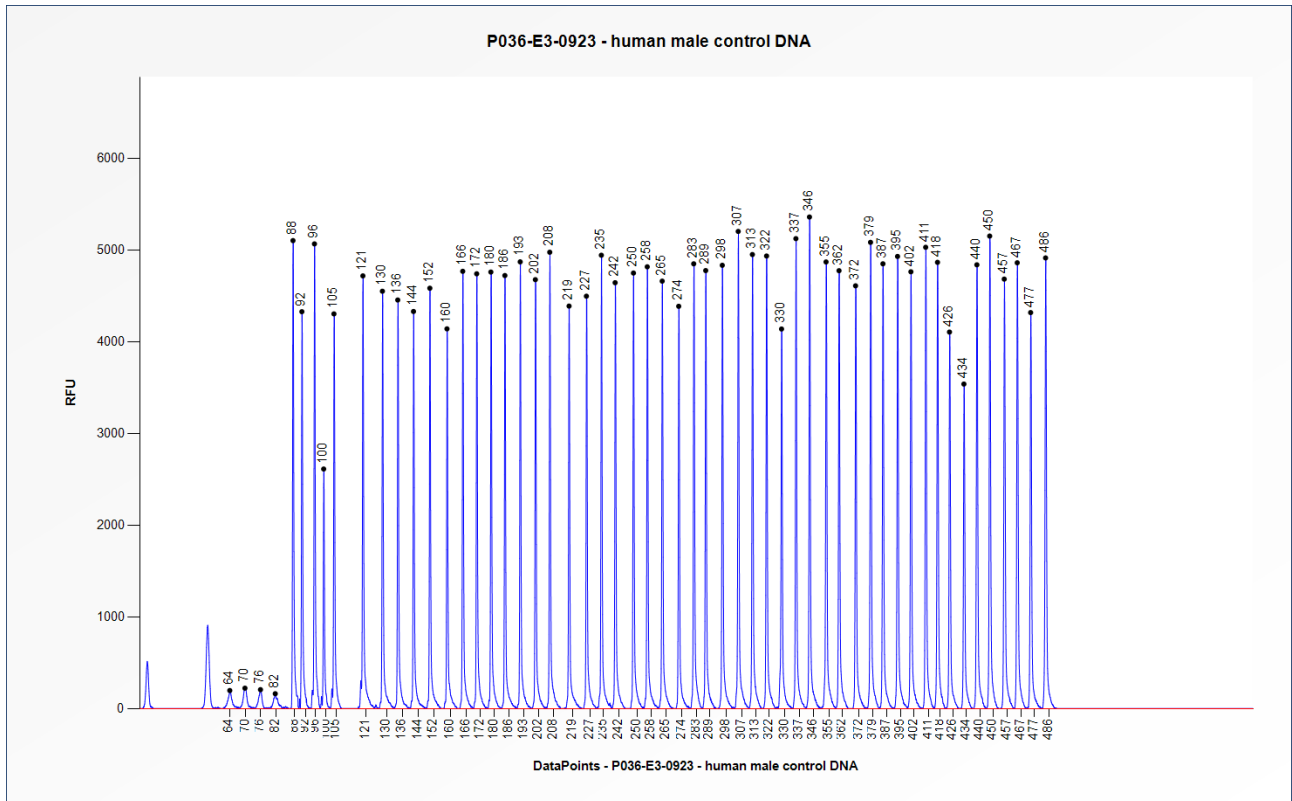
Figure 1. Capillary electrophoresis pattern from a sample of approximately 50 ng human male control DNA analysed with SALSA MLPA Probemix P036 Subtelomeres Mix 1 (E3-0923).
