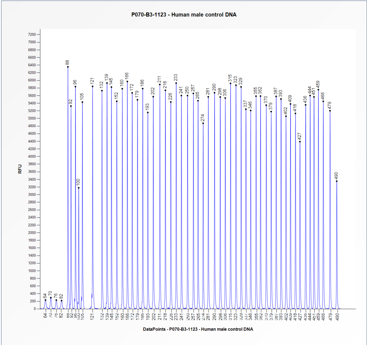
Figure 1. Capillary electrophoresis pattern from a sample of approximately 50 ng human male control DNA analysed with SALSA MLPA Probemix P070 Subtelomeres Mix 2B (B3-1123).
