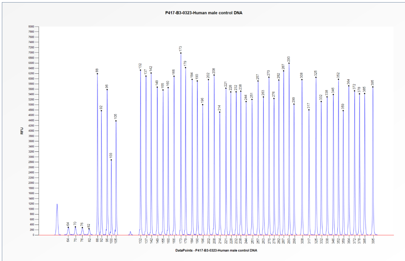
Figure 1. Capillary electrophoresis pattern from a sample of approximately 50 ng human male control DNA analysed with SALSA MLPA Probemix P417 BAP1 (B3-0323).
