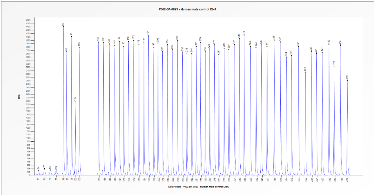
Figure 1. Capillary electrophoresis pattern from a sample of approximately 50 ng human male control DNA analysed with SALSA MLPA Probemix P002 BRCA1 (D1-0823).
