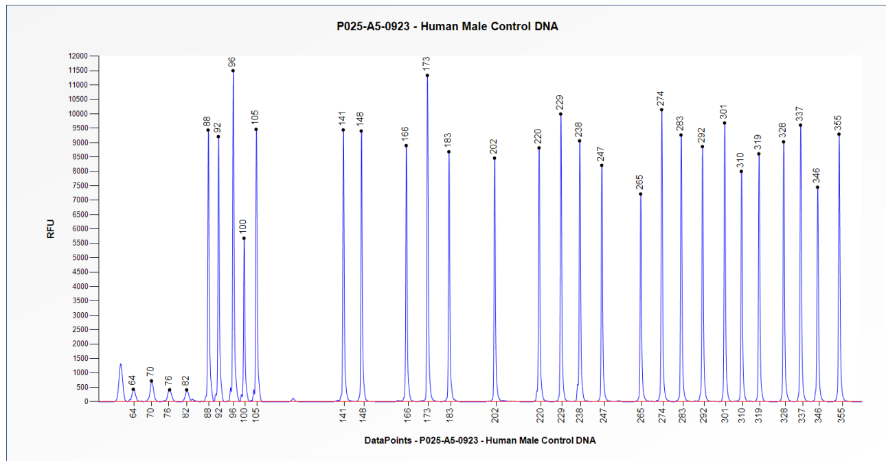
Figure 1. Capillary electrophoresis pattern from a sample of approximately 50 ng human male control DNA analysed with SALSA MLPA Probemix P025 Canavan disease (A5-0923).
