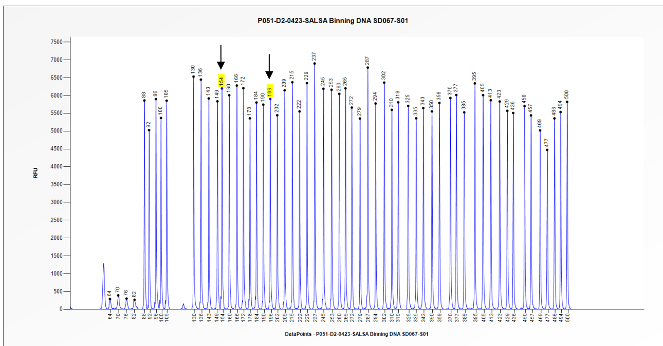
Figure 2. Capillary electrophoresis pattern from SALSA Binning DNA SD067-S01 (approximately 50 ng) analysed with SALSA MLPA Probemix P051 Parkinson mix 1 (D2-0423). The location of the SNCA A30P-specific probe at 154 nt and LRK2 G2019S-specific probe at 196 nt is indicated.
