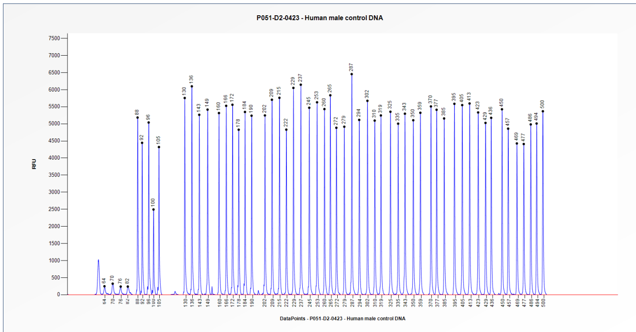
Figure 1. Capillary electrophoresis pattern from a sample of approximately 50 ng human male control DNA analysed with SALSA MLPA Probemix P051 Parkinson mix 1 (D2-0423).
