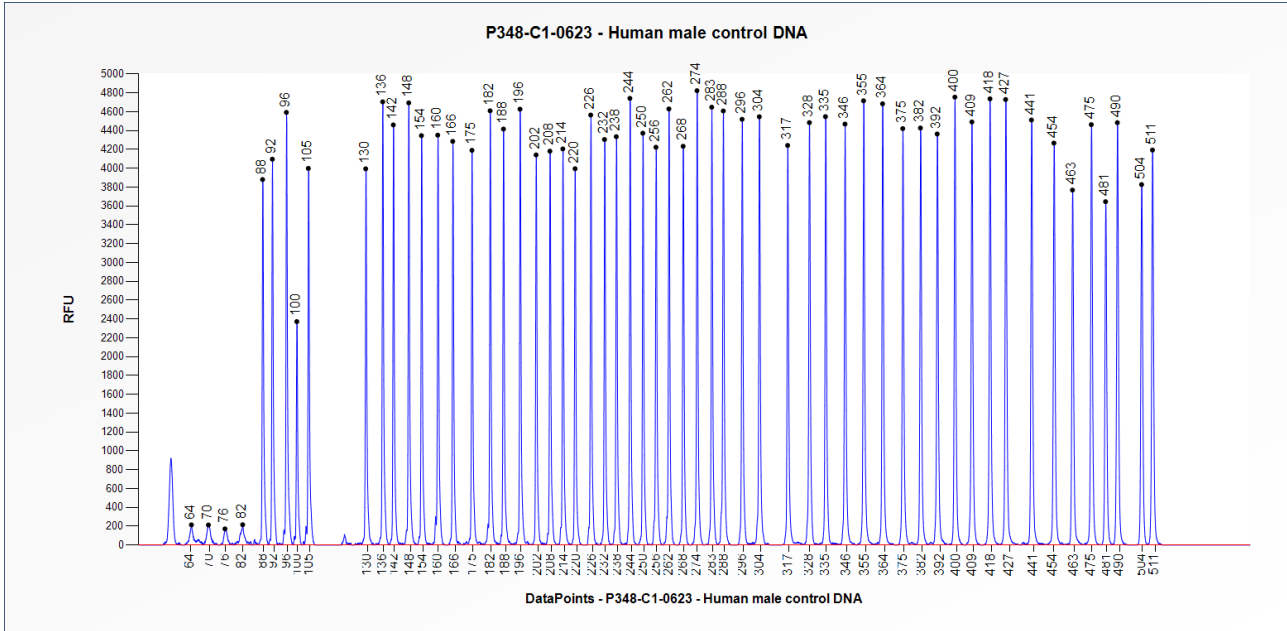
Figure 1. Capillary electrophoresis pattern from a sample of approximately 50 ng human male control DNA analysed with SALSA MLPA Probemix P348 ATP1A2-CACNA1A-PRRT2 (C1-0623).
