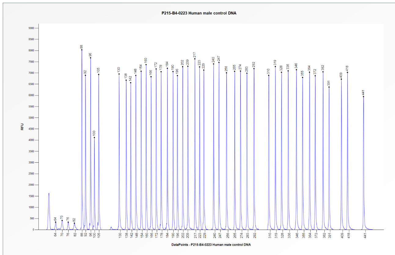
Figure 1. Capillary electrophoresis pattern from a sample of approximately 50 ng human male control DNA analysed with SALSA MLPA Probemix P215 EXT (B4-0223).
