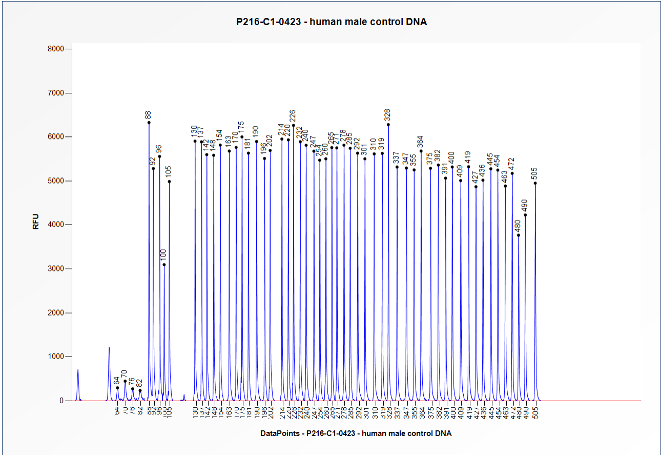
Figure 1. Capillary electrophoresis pattern from a sample of approximately 50 ng human male control DNA analysed with SALSA MLPA Probemix P216 Growth Hormone Deficiency (C1-0423).
