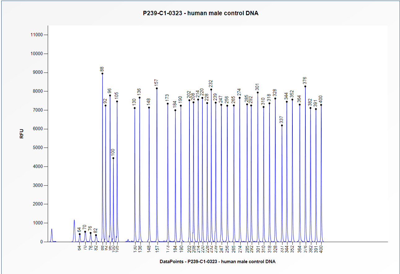
Figure 1. Capillary electrophoresis pattern from a sample of approximately 50 ng human male control DNA analysed with SALSA MLPA Probemix P239 BRCA1 region (C1-0323).
