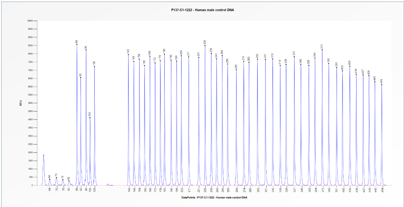
Figure 1. Capillary electrophoresis pattern from a sample of approximately 50 ng human male control DNA analysed with SALSA MLPA Probemix P137 SCN1A (C1-1222).
