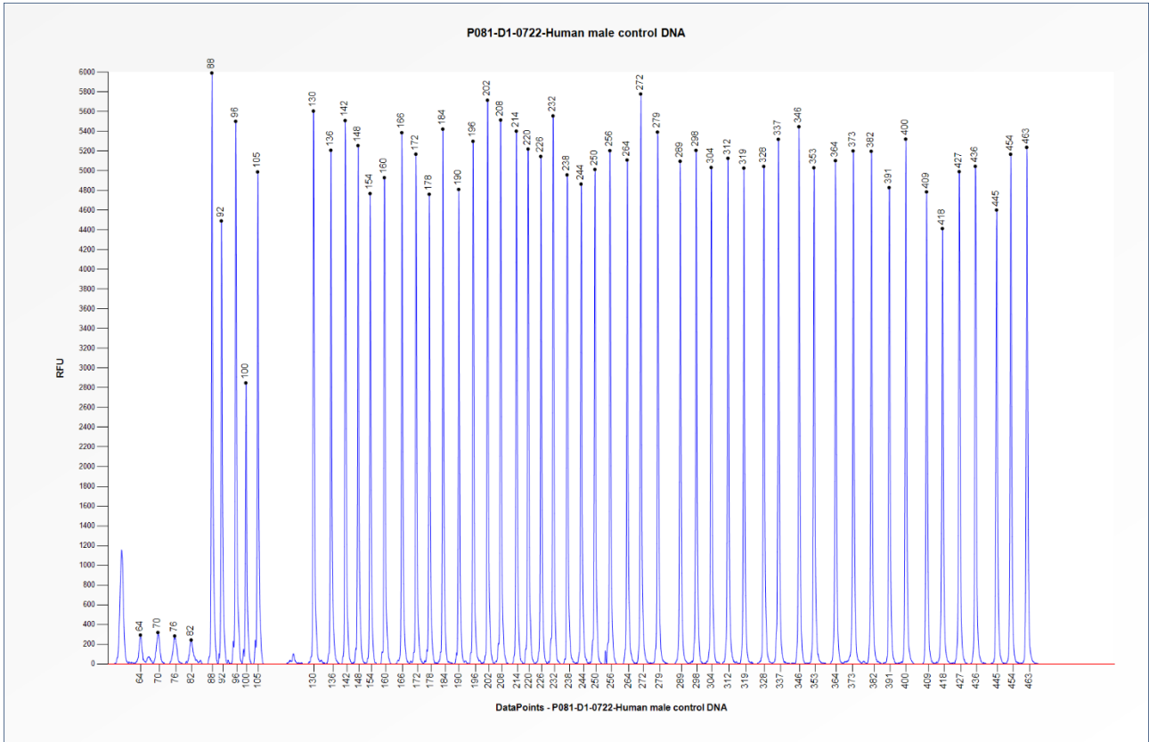
Figure 1. Capillary electrophoresis pattern from a sample of approximately 50 ng human male control DNA analysed with SALSA MLPA Probemix P081 NF1 mix 1 (D1-0722).
