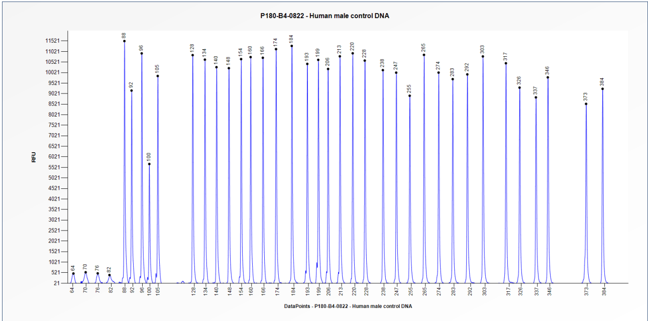
Figure 1. Capillary electrophoresis pattern from a sample of approximately 50 ng human male control DNA analysed with SALSA MLPA Probemix P180 Limb Malformations-2 (B4-0822).
