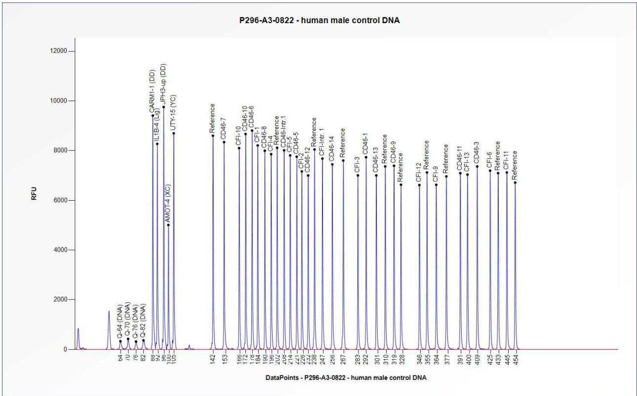
Figure 1. Capillary electrophoresis pattern from a sample of approximately 50 ng human male control DNA analysed with SALSA MLPA Probemix P296 aHUS (A3-0822).
