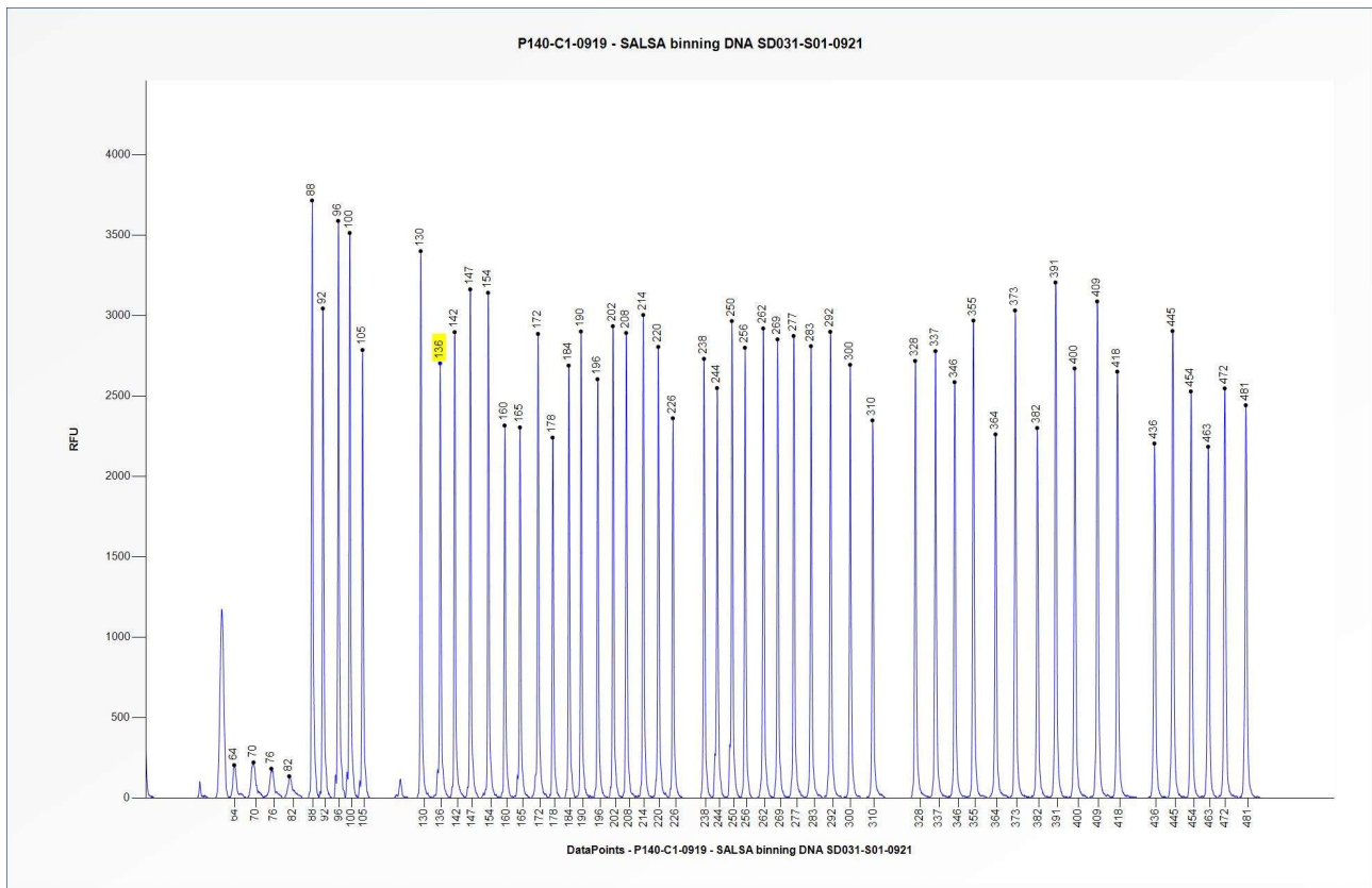
Figure 1. Capillary electrophoresis pattern from SALSA Binning DNA SD031-S01-0921 (approximately 50 ng) analysed with SALSA MLPA Probemix P140 HBA (C1-0919). The location of the Hb Constant Spring mutation-specific probe at 136 nt is indicated. Probe peak heights may vary between different lots of the P140-C1 probemix.
