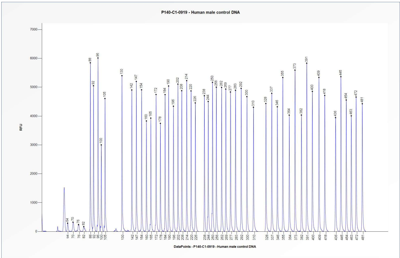
Figure 2. Capillary electrophoresis pattern from a sample of approximately 50 ng human male control DNA analysed with SALSA MLPA Probemix P140 HBA (C1-0919). Probe peak heights may vary between different lots of the P140-C1 probemix.
