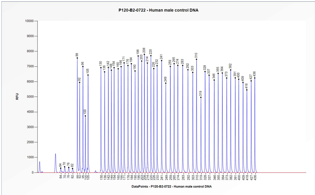
Figure 1. Capillary electrophoresis pattern from a sample of approximately 50 ng human male control DNA analysed with SALSA MLPA Probemix P120 PANK2/PLA2G6 (B2-0722).
