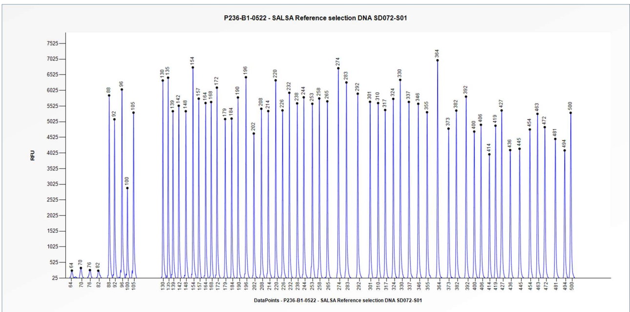
Figure 2. Capillary electrophoresis pattern from SALSA Reference Selection DNA SD072-S01 (approximately 50 ng) analysed with SALSA MLPA Probemix P236 CFH Region (B1-0522).
