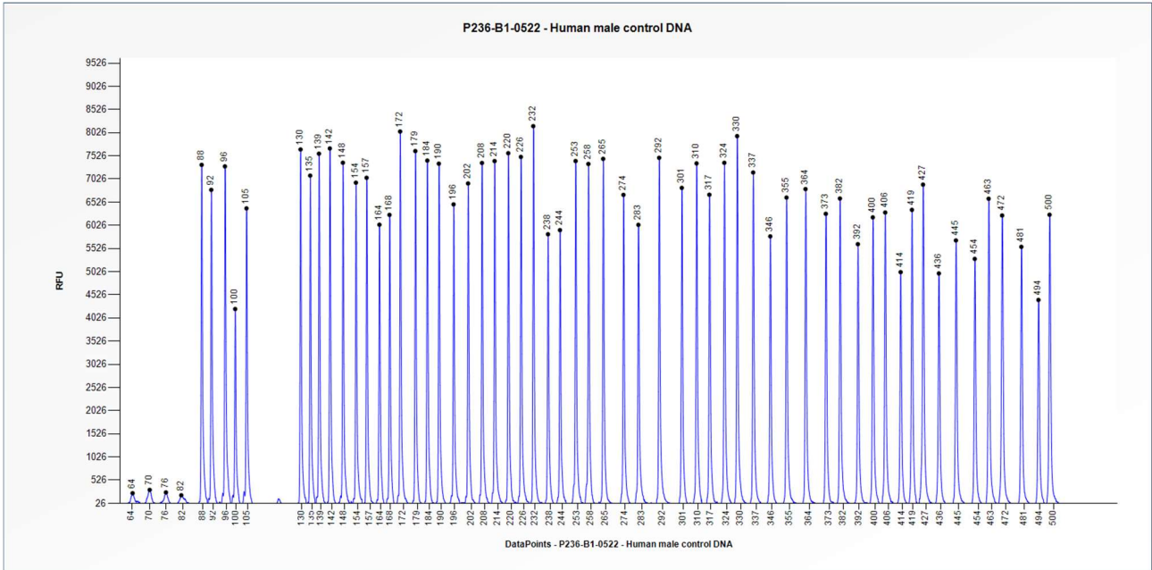
Figure 1. Capillary electrophoresis pattern from a sample of approximately 50 ng human male control DNA analysed with SALSA MLPA Probemix P236 CFH Region (B1-0522).
