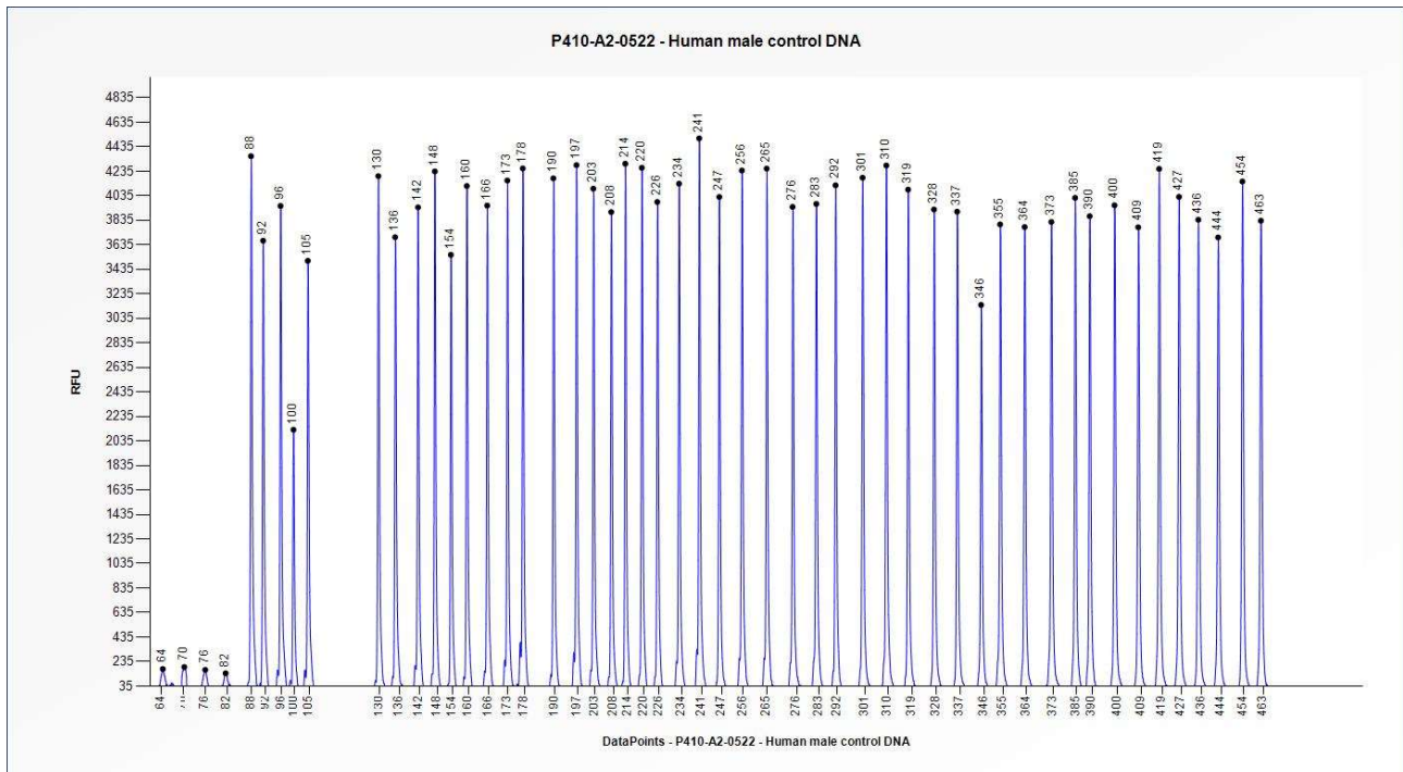
Figure 1. Capillary electrophoresis pattern from a sample of approximately 50 ng human male control DNA analysed with SALSA MLPA Probemix P410 GRIN2A-GRIN2B (A2-0522).
