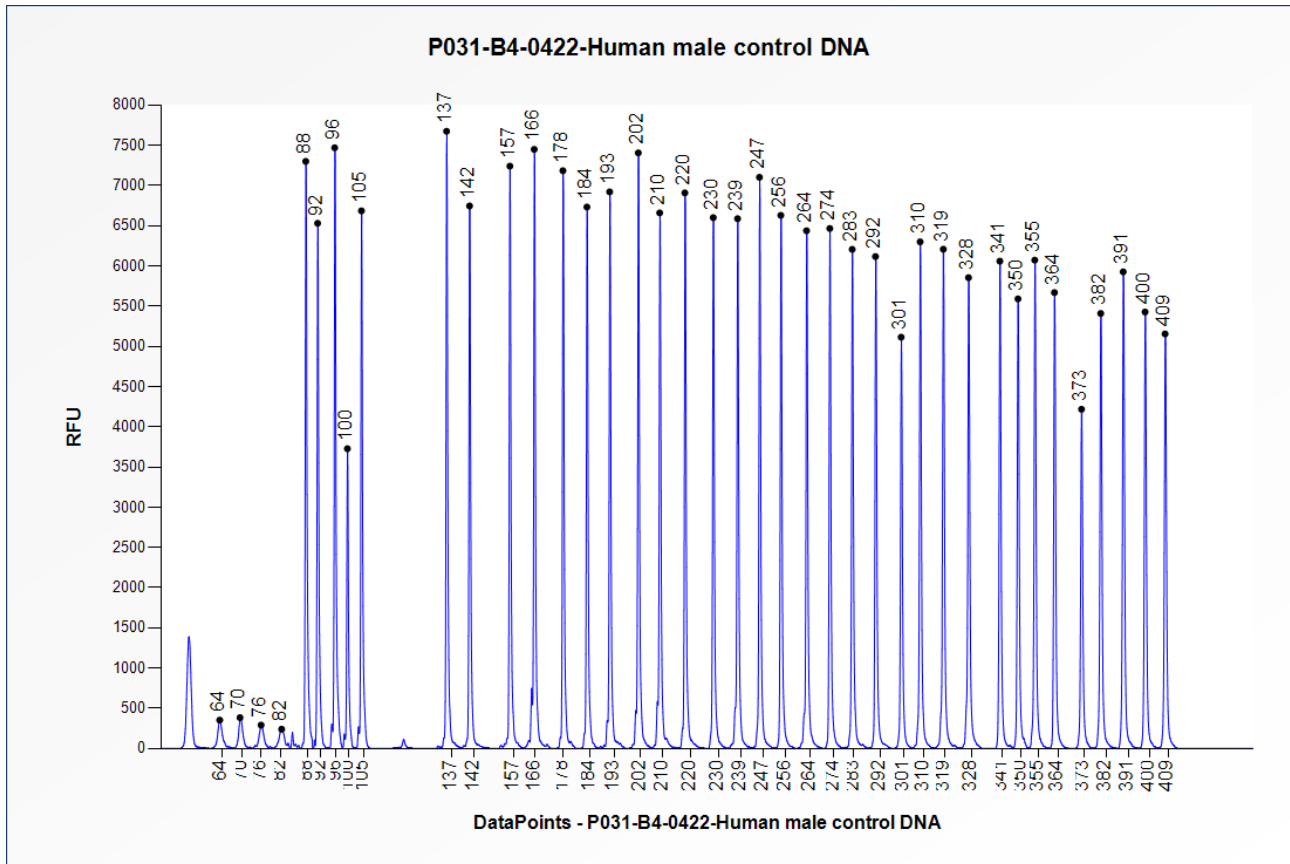
Figure 1. Capillary electrophoresis pattern from a sample of approximately 50 ng human male control DNA analysed with SALSA MLPA Probemix P031 FANCA mix 1 (B4-0422).
