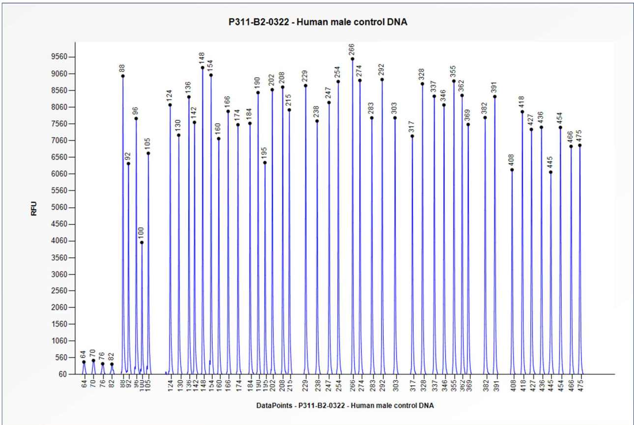
Figure 1. Capillary electrophoresis pattern from a sample of approximately 50 ng human male control DNA analysed with SALSA MLPA Probemix P311 CHD (B2-0322).
