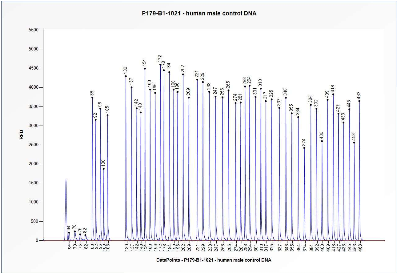
Figure 1. Capillary electrophoresis pattern from a sample of approximately 50 ng human male control DNA analysed with SALSA MLPA Probemix P179 Limb malformations-1 (B1-1021).
