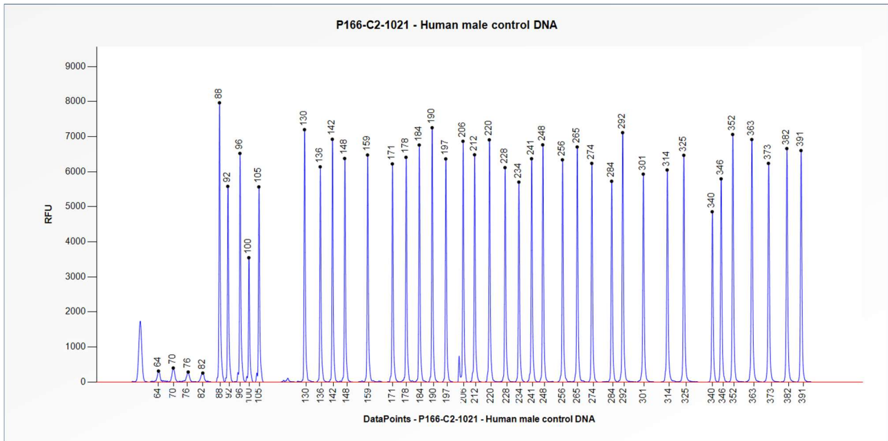
Figure 1. Capillary electrophoresis pattern from a sample of approximately 50 ng human male control DNA analysed with SALSA MLPA Probemix P166 KCNQ2 (C2-1021).
