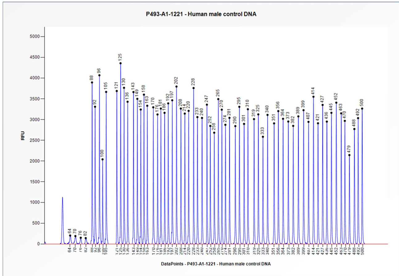
Figure 1. Capillary electrophoresis pattern from a sample of approximately 50 ng human male control DNA analysed with SALSA MLPA Probemix P493 SMCHD1 (A1-1221).
