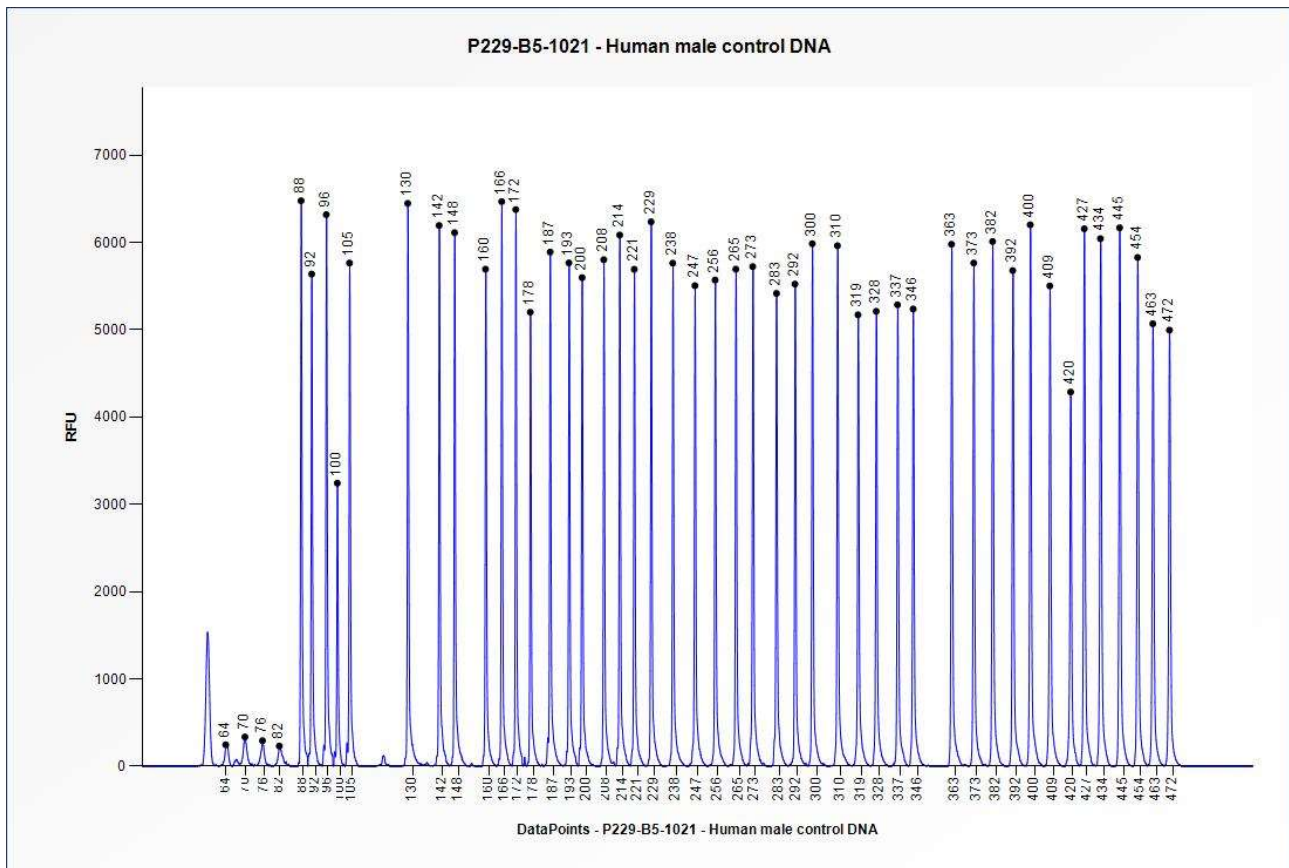
Figure 1. Capillary electrophoresis pattern from a sample of approximately 50 ng human male control DNA analysed with SALSA MLPA Probemix P229 OPA1 (B5-1021).
