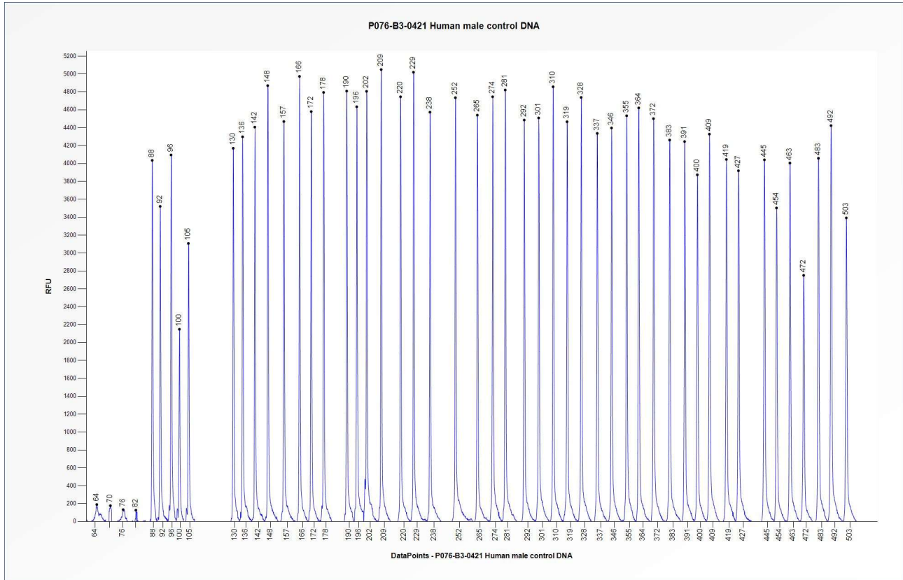
Figure 1. Capillary electrophoresis pattern from a sample of approximately 50 ng human male control DNA analysed with SALSA MLPA Probemix P076 ACADVL-SLC22A5 (B3-0421).
