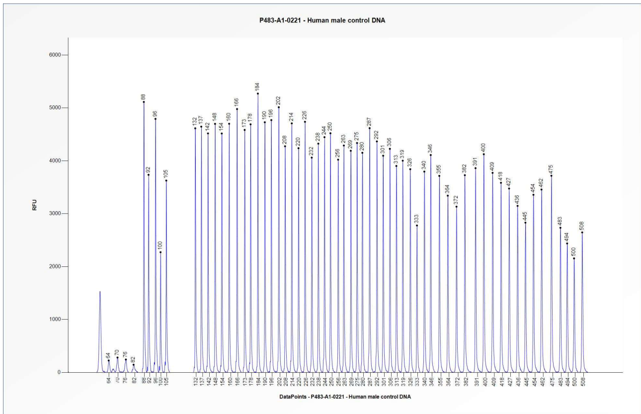
Figure 1. Capillary electrophoresis pattern from a sample of approximately 50 ng human male control DNA analysed with SALSA MLPA Probemix P483 HER gene family (A1-0221).
