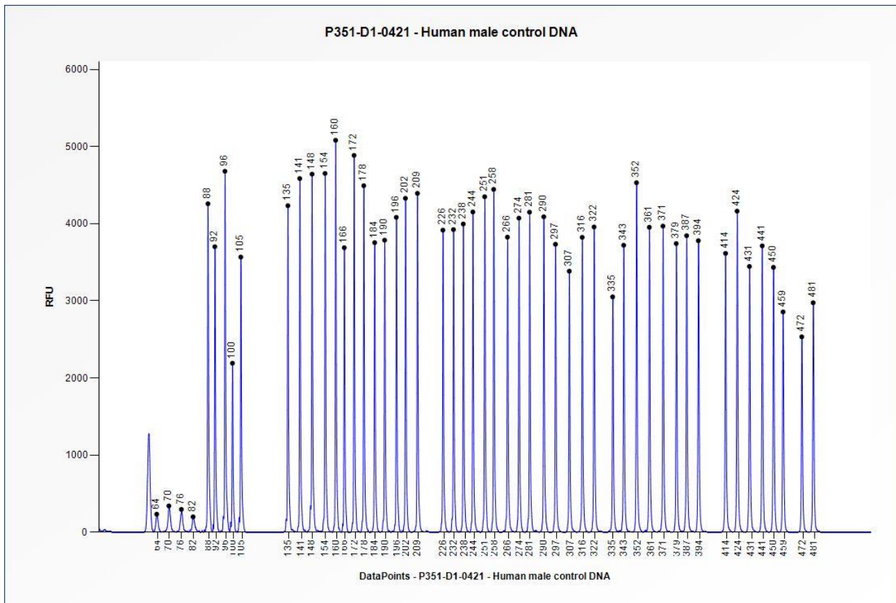
Figure 1. Capillary electrophoresis pattern from a sample of approximately 50 ng human male control DNA analysed with SALSA MLPA Probemix P351 PKD1 (D1-0421).
