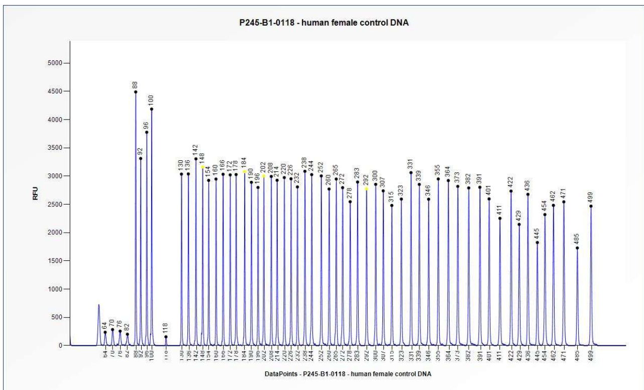
Figure 2. Capillary electrophoresis pattern from a sample of approximately 50 ng human female control DNA analysed with SALSA MLPA Probemix P245 Microdeletion Syndromes-1A (B1-0118).
