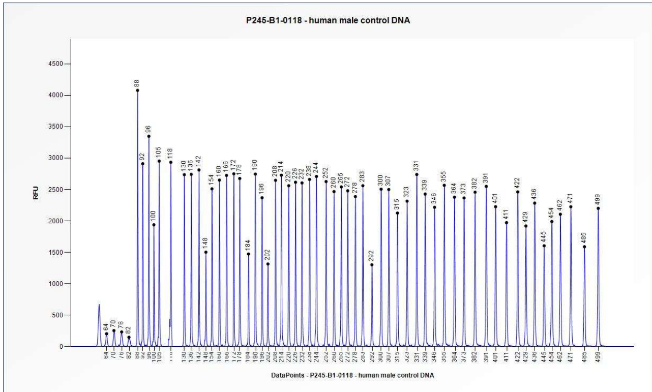
Figure 1. Capillary electrophoresis pattern from a sample of approximately 50 ng human male control DNA analysed with SALSA MLPA Probemix P245 Microdeletion Syndromes-1A (B1-0118).
