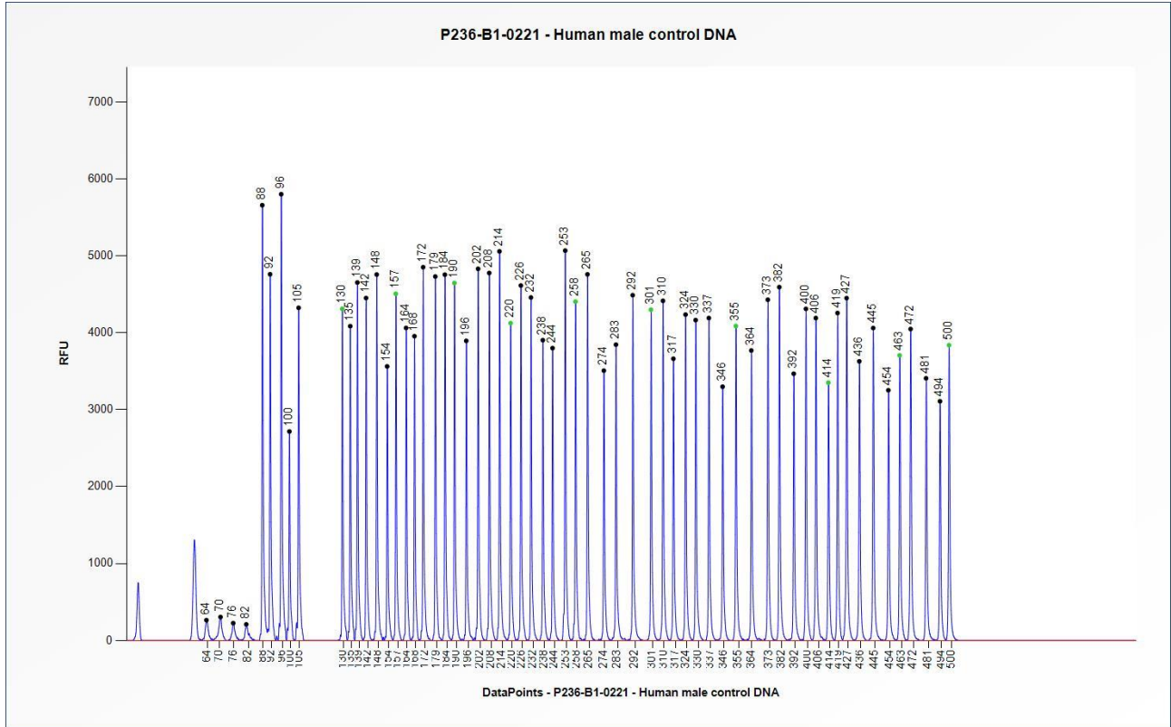
Figure 1. Capillary electrophoresis pattern from a sample of approximately 50 ng human male control DNA analysed with SALSA MLPA Probemix P236 CFH Region (B1-0221).
