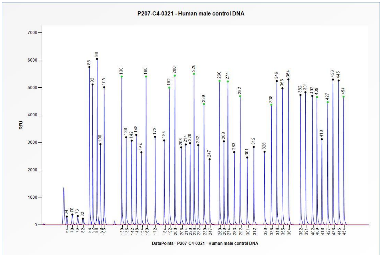
Figure 1. Capillary electrophoresis pattern from a sample of approximately 50 ng human male control DNA analysed with SALSA MLPA Probemix P207 F9 (C4-0321).
