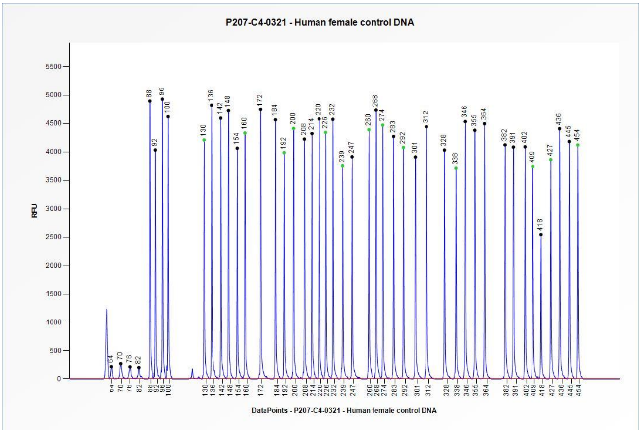
Figure 2. Capillary electrophoresis pattern from a sample of approximately 50 ng human female control DNA analysed with SALSA MLPA Probemix P207 F9 (C4-0321).
