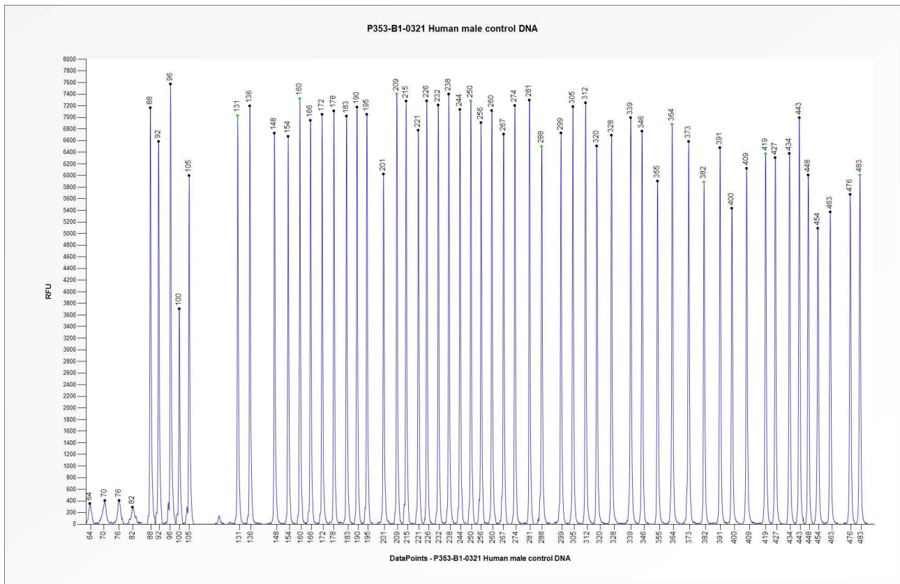
Figure 1. Capillary electrophoresis pattern from a sample of approximately 50 ng human male control DNA analysed with SALSA MLPA Probemix P353 CMT4 (B1-0321).
