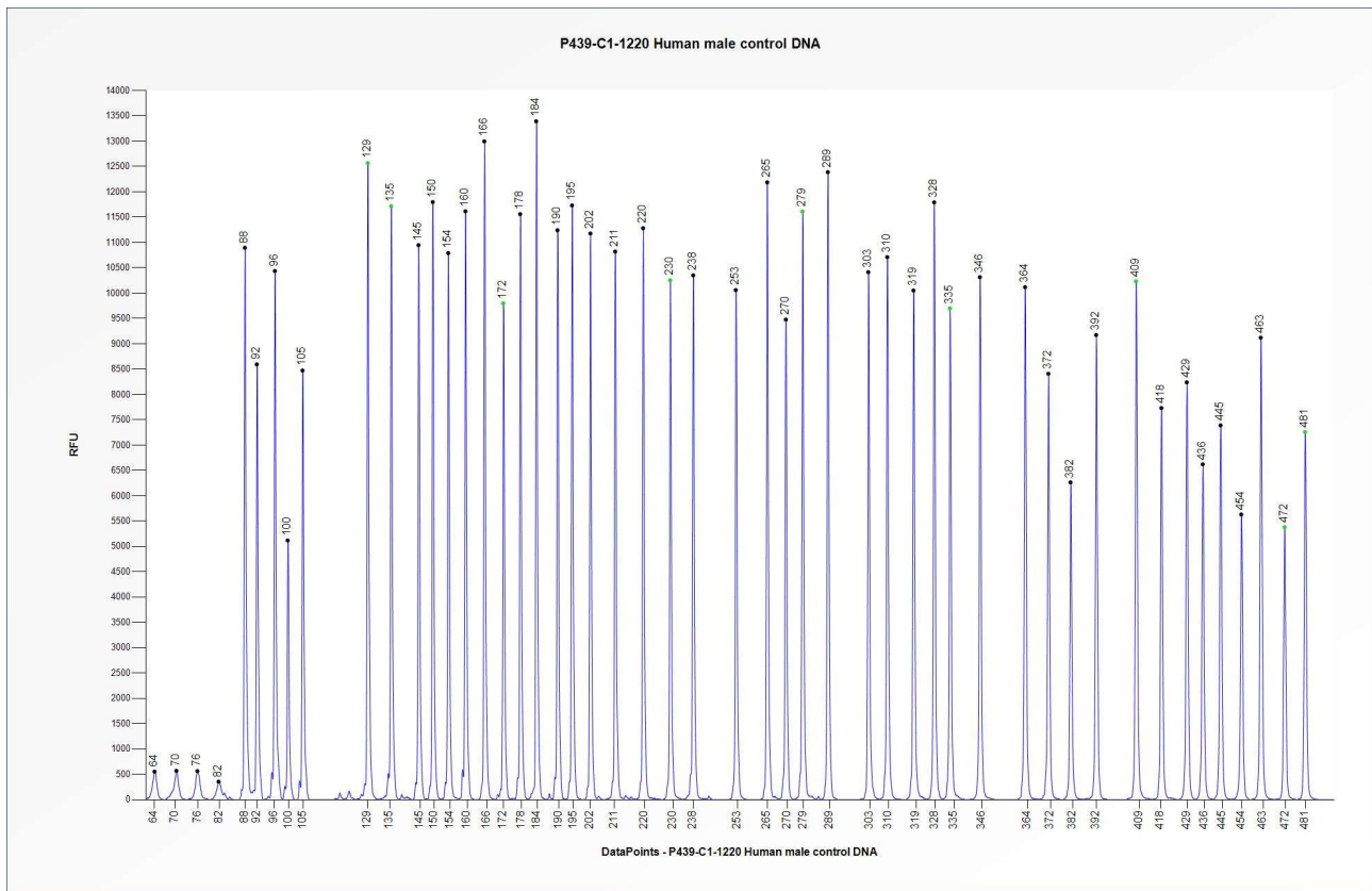
Figure 1. Capillary electrophoresis pattern from a sample of approximately 50 ng human male control DNA analysed with SALSA MLPA Probemix P439 COL4A3 (C1-1220).
