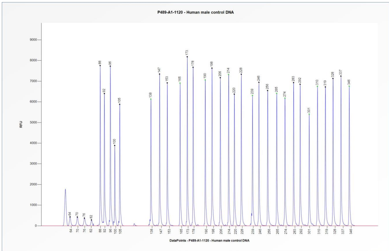
Figure 1. Capillary electrophoresis pattern from a sample of approximately 50 ng human male control DNA analysed with SALSA MLPA Probemix P489 BARD1 (A1-1120).
