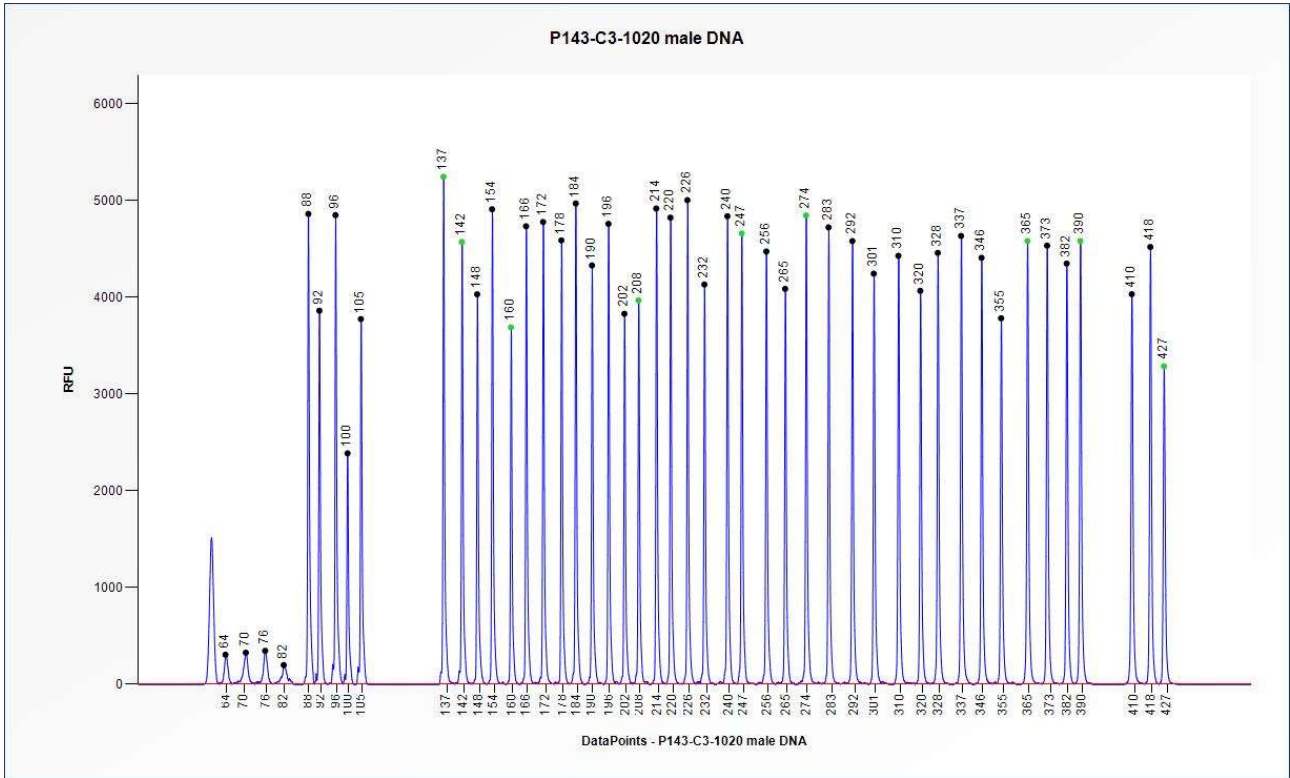
Figure 1. Capillary electrophoresis pattern from a sample of approximately 50 ng human male control DNA analysed with SALSA MLPA Probemix P143 MFN2-MPZ (C3-1020).
