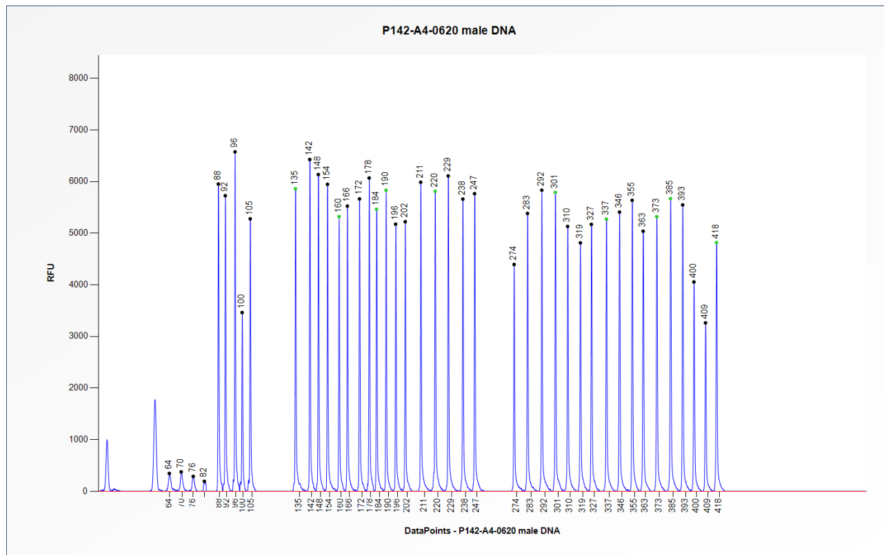
Figure 1. Capillary electrophoresis pattern from a sample of approximately 50 ng human male control DNA analysed with SALSA MLPA Probemix P142 NIPBL-2 (A4-0620).
