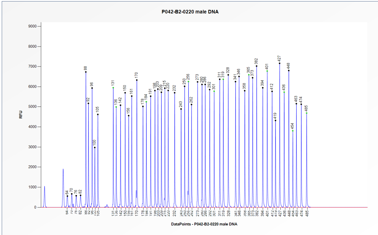
Figure 1. Capillary electrophoresis pattern from a sample of approximately 50 ng human male control DNA analysed with SALSA MLPA Probemix P042 ATM-2 (B2-0220).
